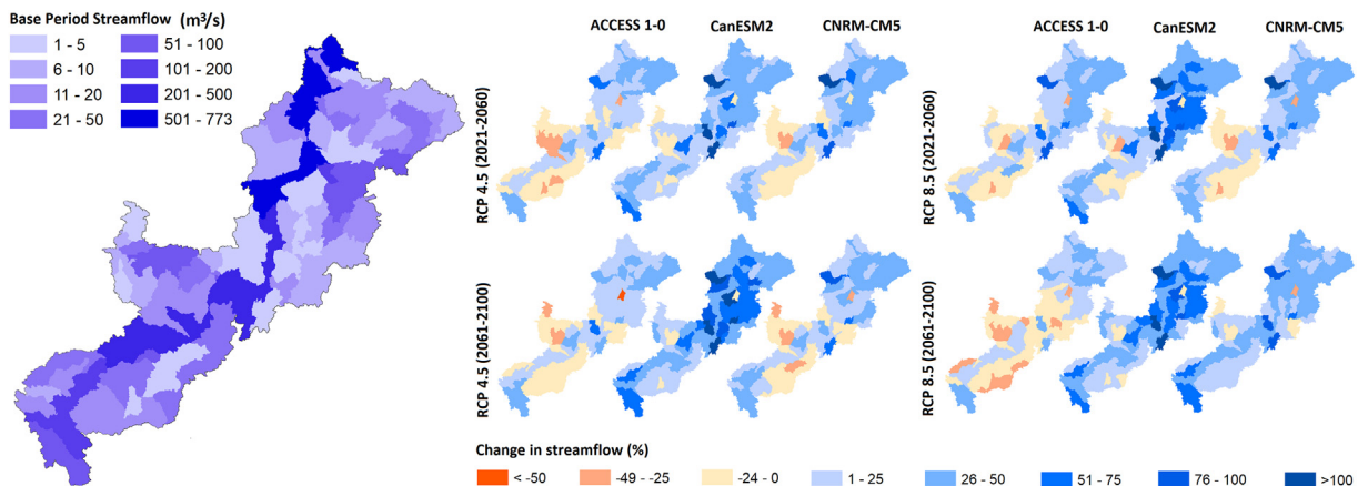
Fig. 2. Annual average streamflow changes (%) in two future periods for two emission scenarios compared to the baseline period ( \text{m}^3/\text{s} ).
